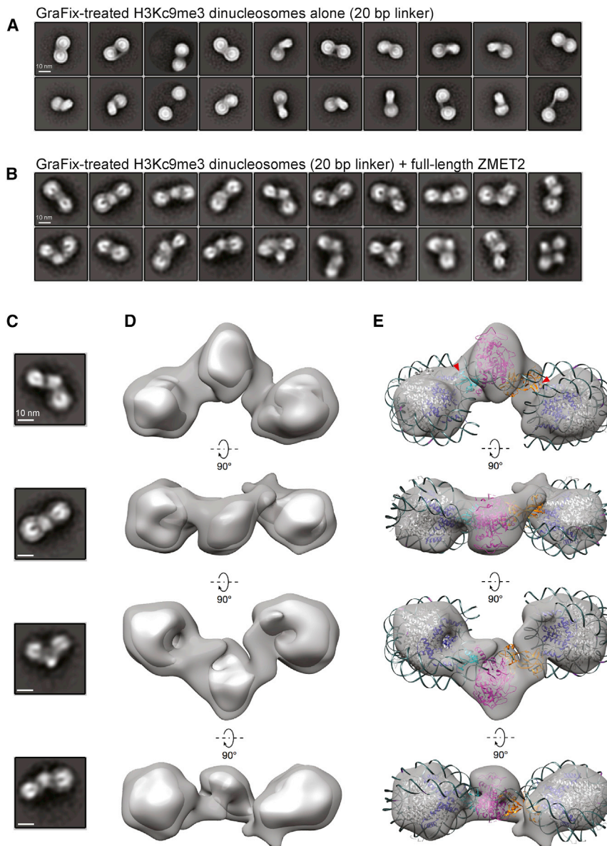
Figure 5. Visualization of ZMET2 Bridging the Dinucleosome by Negative Stain Electron Microscopy
