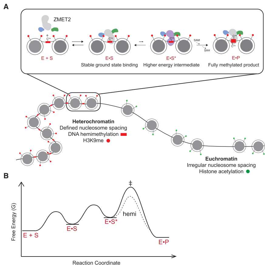
Figure 6. Model for ZMET2 Assembly and Activity on Chromatin
