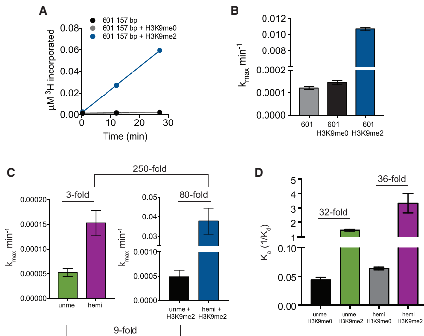
Figure 2. ZMET2 Binding and Activity Are Increased by the H3K9me Mark and DNA Hemimethylation
