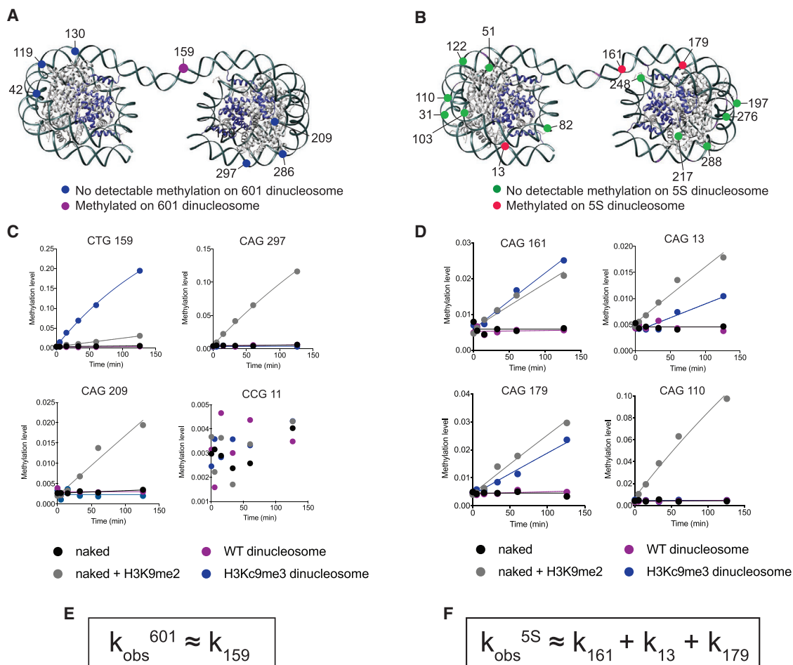
Figure 4. ZMET2 Preferentially Methylates the Linker DNA in H3K9me3 Dinucleosomes
