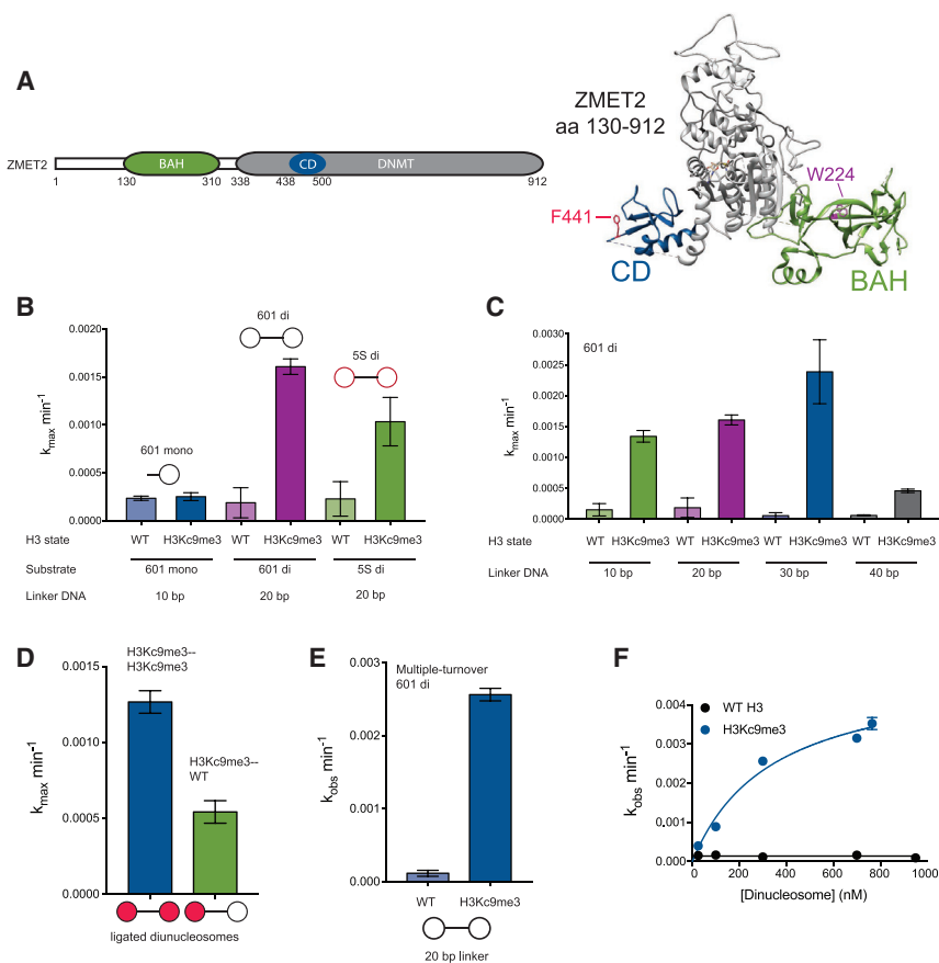
Figure 1. ZMET2 Methylates H3K9me3 Dinucleosomes Faster Than Mononucleosomes
