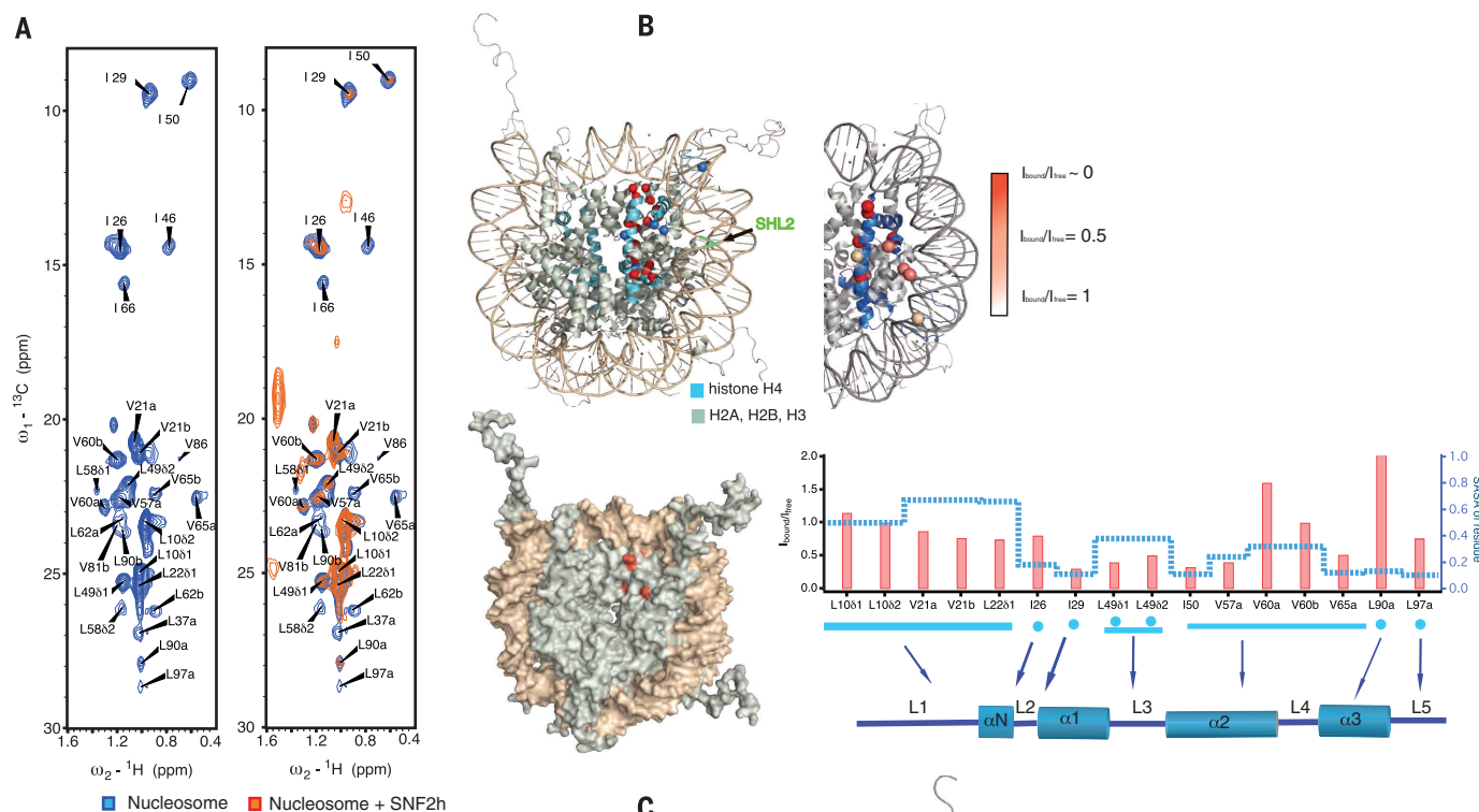
Fig. 1. Methyl-TROSY spectra of nucleosome bound to SNF2h.
