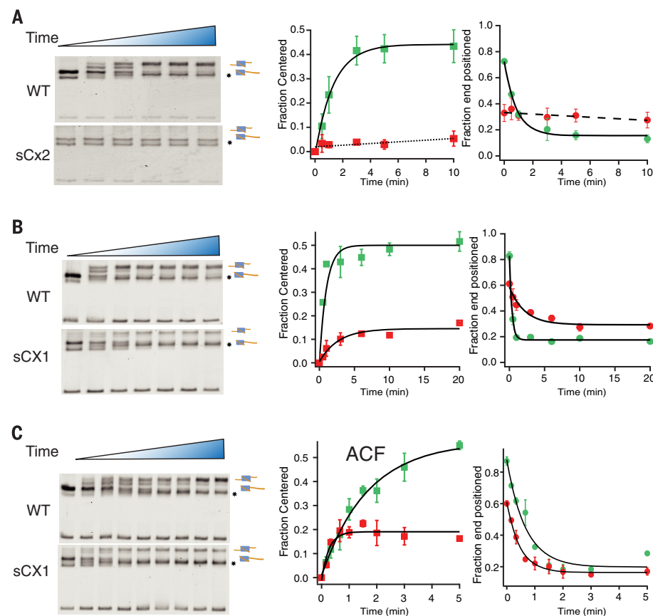
Fig. 3. Investigating the extent of H3-H4 flexibility required for remodeling by SNF2h and ACF.
