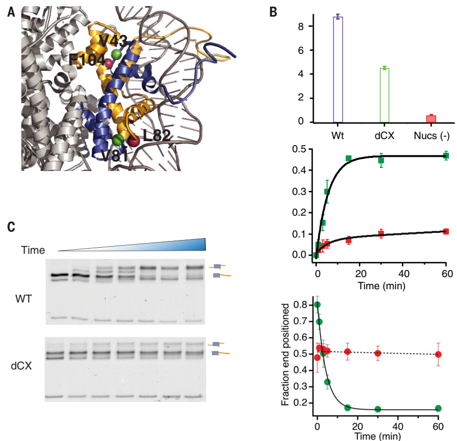
Fig. 2. Functional impact of restricting H3-H4 interface on SNF2h. (A) Location of residues mutated to cysteines. Residues L82 and F104 in H3, and V43 and V81 in H4, were mutated to Cys. (B) Comparison of SNF2h ATPase rates in the presence of WT (purple), dCX (green), and no nucleosomes (red). Error bars represent the SDs from three independent experiments. (C) Comparison of remodeling of WT and dCX nucleosomes by SNF2h. Left panels: representative gel for remodeling kinetics for WT (top panel) and dCX (bottom panel), respectively. Right panels: Quantification of the fraction of centered nucleosomes (top panel) and the fraction of end-positioned nucleosomes (bottom panel) as a function of time. WT data are in green and dCX data are in red. Time points (in minutes): 0, 1, 3, 5, 10, 20, and 60. Error bars are the SDs from three independent experiments. In the top right panel, the observed rate constant, k_{obs} , for the WT is 0.18 \pm 0.03 \text{ min}^{-1} . The rate constant for the minor fast phase of dCX ( k_{1fixed} ) was fixed to be the same as the k_{obs} for the WT. The rate constant for the major slow phase ( k_{2obs} ) with the constraint of k_{1fixed} = 0.18 \text{ min}^{-1} was calculated to be 0.003 \pm 0.001 \text{ min}^{-1} . Fitting the entire time course for dCX to a single exponential gives a value of k_{obs} = 0.01 \pm 0.001 \text{ min}^{-1} . For all experiments with cysteine cross-linked nucleosomes, Cy3-labeled 601+60 DNA was externally added to the WT nucleosome samples to make the reaction conditions between the WT and cross-linked nucleosomes comparable to those of the cross-linked nucleosomes with some free DNA. The free DNA inhibits rates of remodeling in a dose-dependent manner (see supplementary methods for details).
