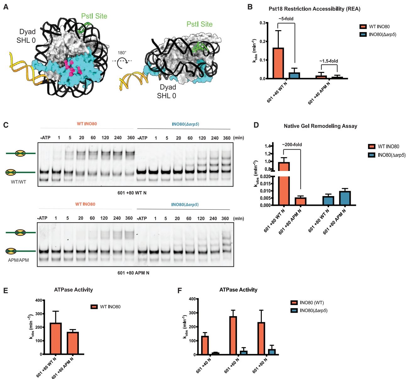
Figure 5. The Arp5 module interacts with the acidic patch to regulate INO80 sliding
